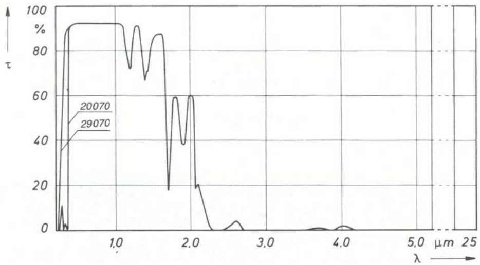
Fig. 16 Spectral Transmission of DEC colorless sheet (Approximation only) (UV to the non-penetrating infrared wavelengths)
