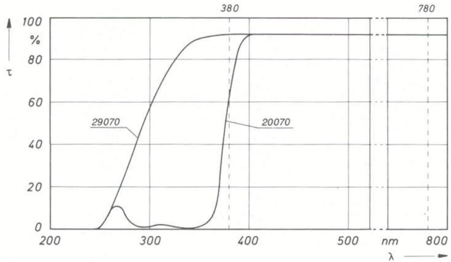
Fig. 15 Comparison of colorless DEC® UVT and UVA sheet (29070 is the UV-transmitting grade & 20070 the UV- absorbing grade)
